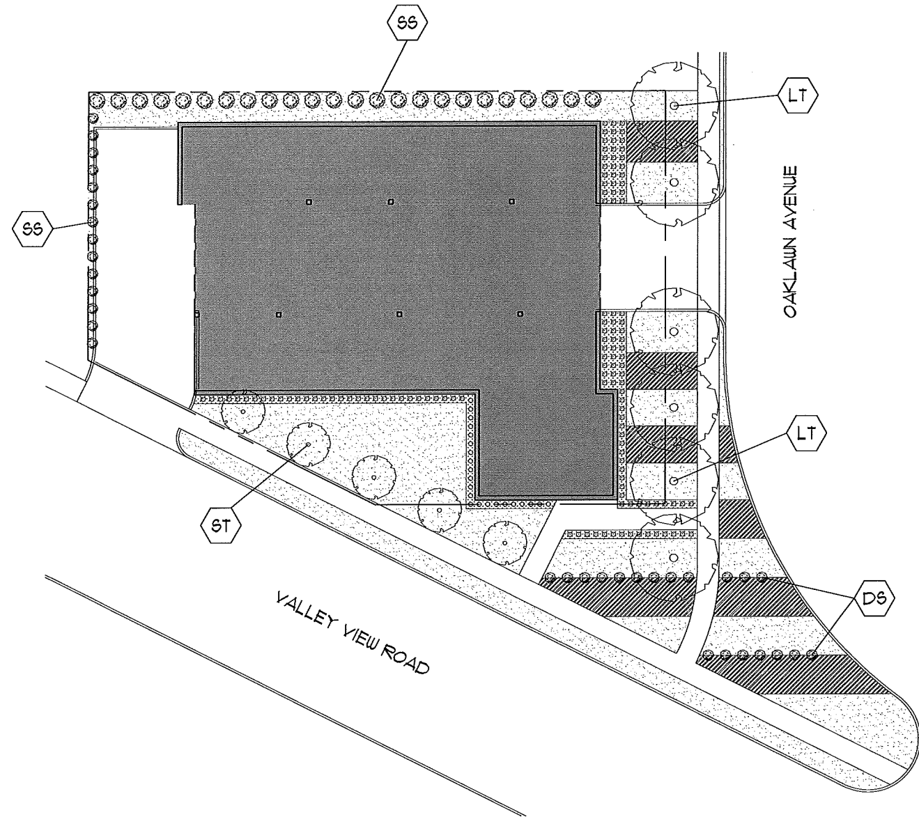
1 LANDSCAPE PLAN AL-1 1" = 30'-0"
